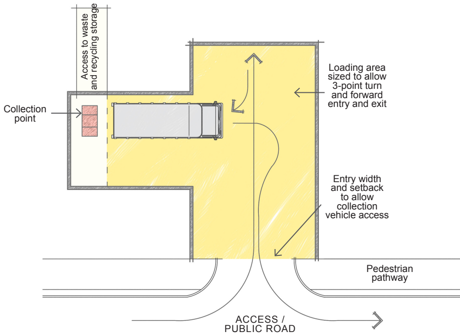
Figure 4.3: Example where reversing has been minimised for on-property collection. This example illustrates that design of these areas need to provide adequate space to allow entry, exit and manoeuvring of the collection vehicle, and also ensure proper clearances at entry/exit point and in the loading area.
